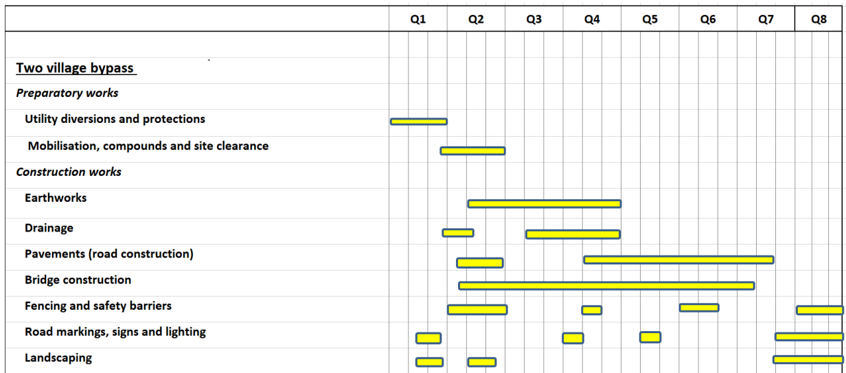
Plate 2.1: Anticipated construction sequence
